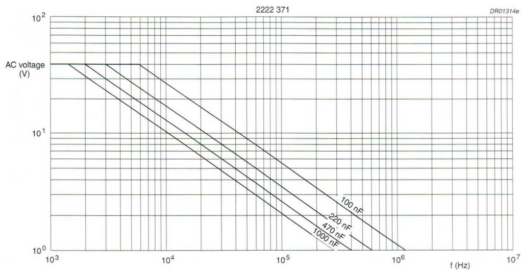
Fig.25 AC voltage (RMS value) as a function of frequency at T_{amb} \leq 85^\circ\text{C} for U_{Rdc} = 63\text{ V} .
