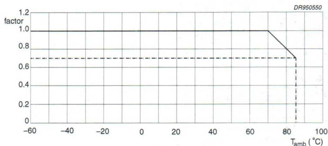
Fig.14 Multiplying factor as a function of temperature.
