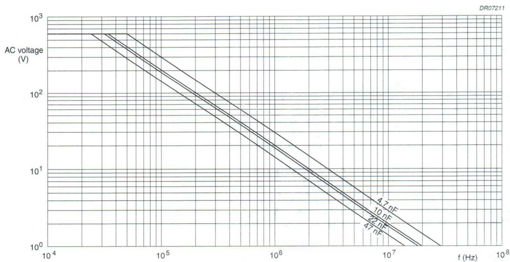
Fig.19 AC voltage (RMS value) as a function of frequency at T_{\text{amb}} \leq 70^\circ\text{C} for U_{\text{Rdc}} = 2000\text{ V} .
