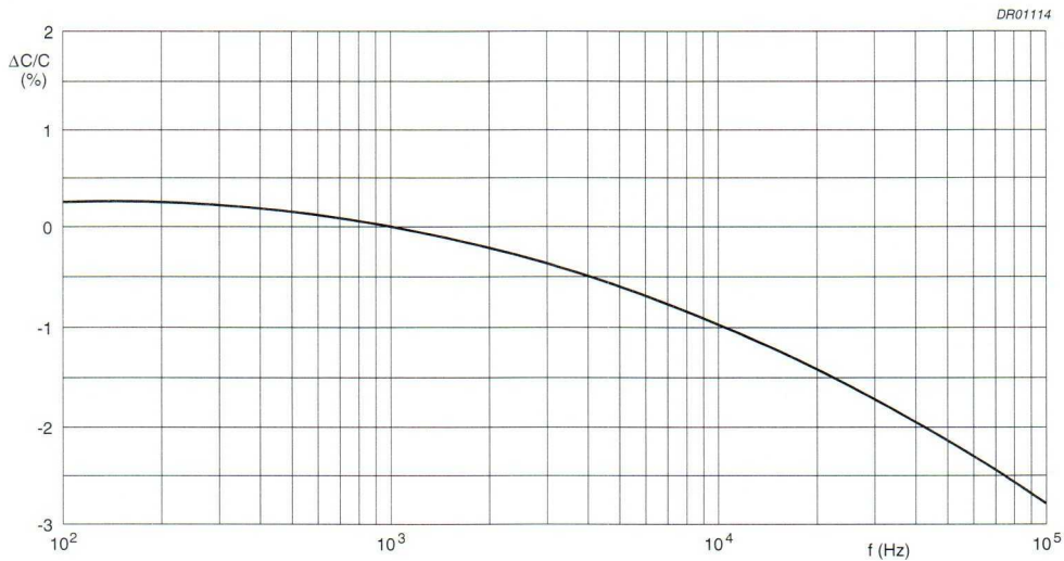
Fig.22 Capacitance change as a function of frequency; typical curve.
