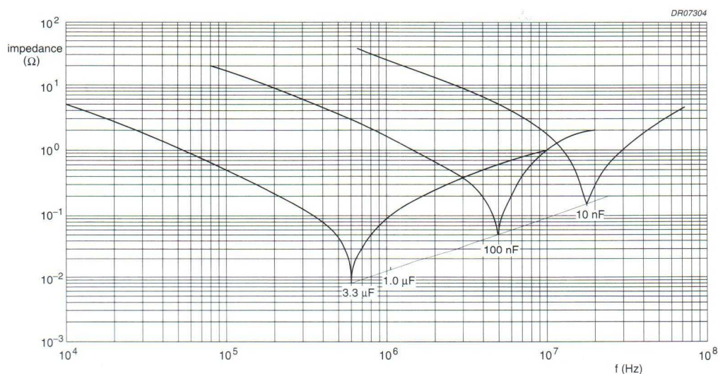
Fig.18 Impedance as a function of frequency; typical curves.
