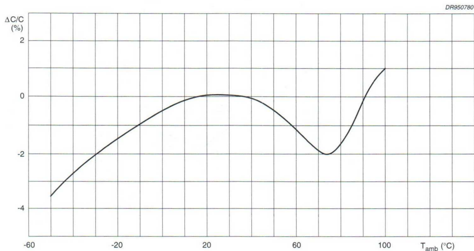
Fig.7 Capacitance change as a function of ambient free air temperature; typical curve.
