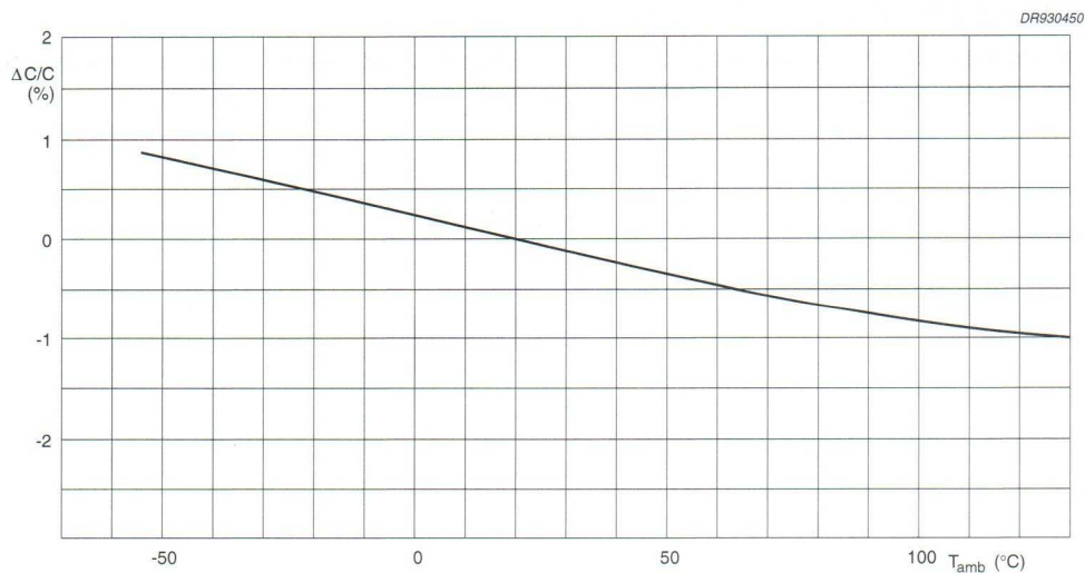
Fig.9 Capacitance change as a function of ambient temperature; typical curve.
