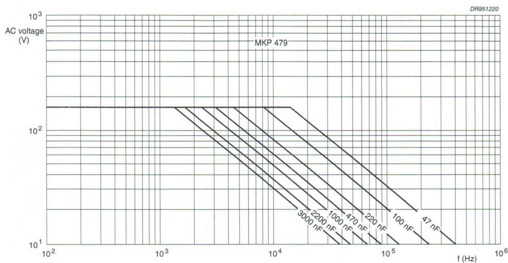
Fig.14 AC voltage (RMS value) as a function of frequency at T_{amb} \leq 70^\circ\text{C} for U_{Rdc} = 250\text{ V} .
