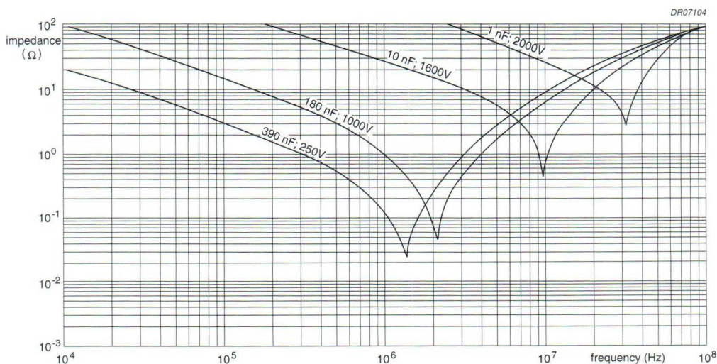
Fig.10 Impedance as a function of frequency; typical curves.
