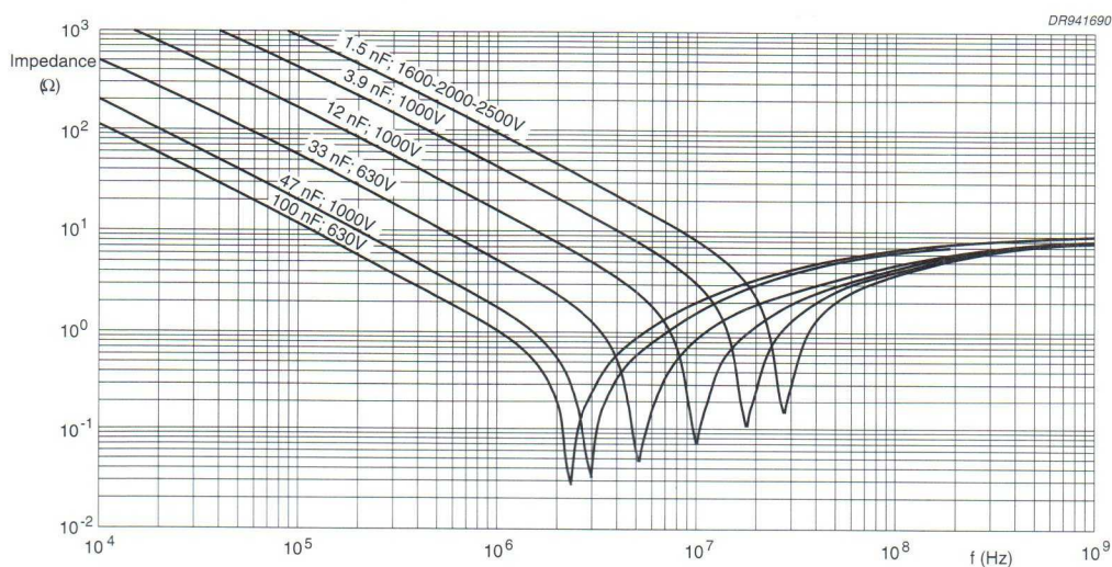
Fig.16 Impedance as a function of frequency; typical curves.
