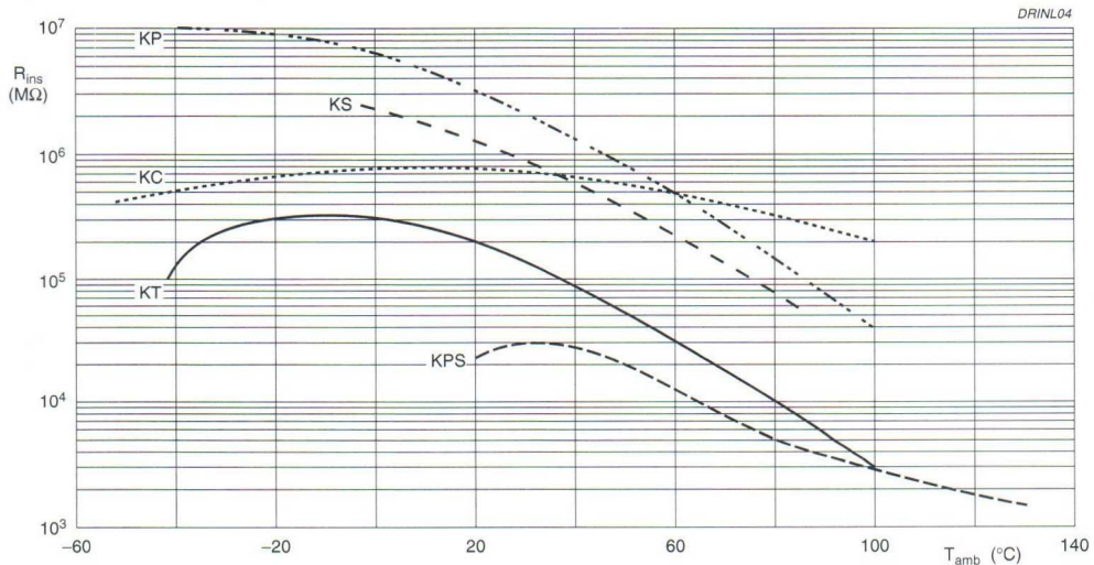
Fig.4 Insulation resistance as a function of ambient free air temperature; typical curves.
