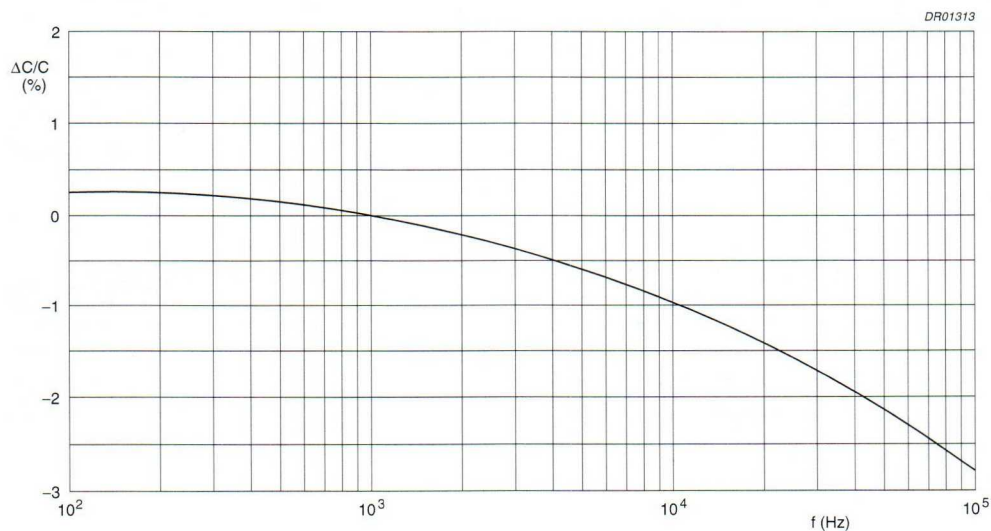
Fig.18 Capacitance change as a function of frequency; typical curve.
