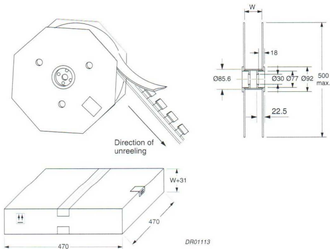
Fig.35 Outlines of reel. Styles: 368, 369, 375, 467, 468 and 479.
