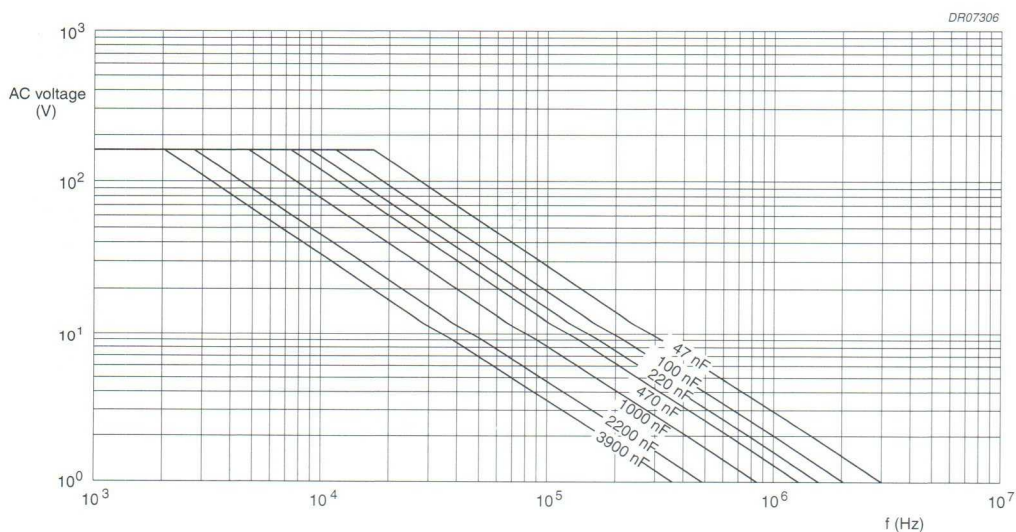
Fig.23 AC voltage (RMS value) as a function of frequency at T_{\text{amb}} \leq 70^\circ\text{C} for U_{\text{Rdc}} = 250\text{ V} .
