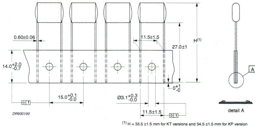
Fig.5 Outline of radial taped capacitors.
