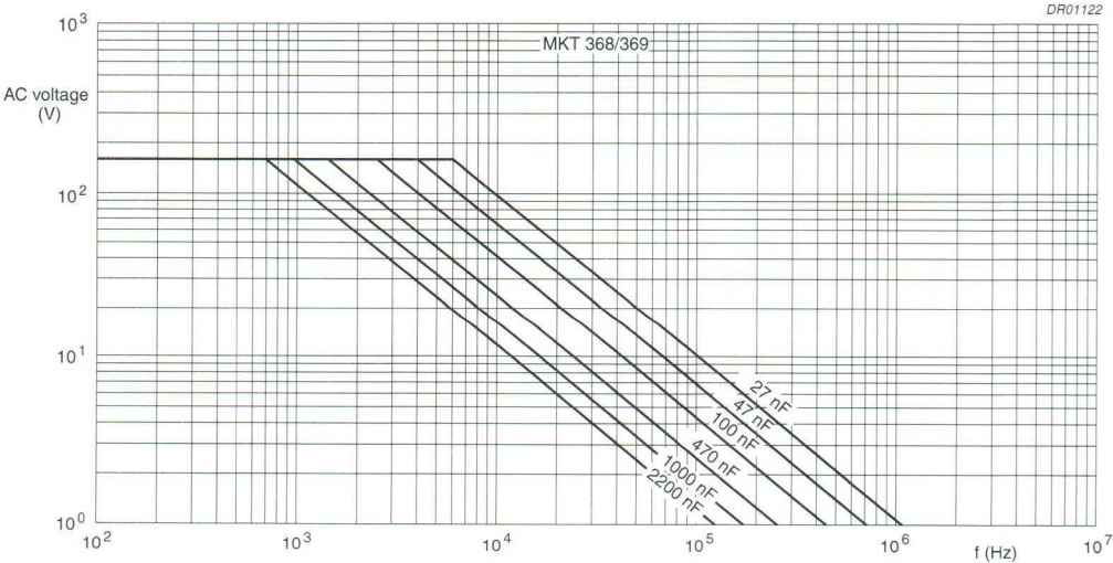
Fig.40 AC voltage (RMS value) as a function of frequency at T_{amb} \leq 85^\circ\text{C} , for U_{Rdc} = 250\text{ V} (2222 368 and 369 styles).
