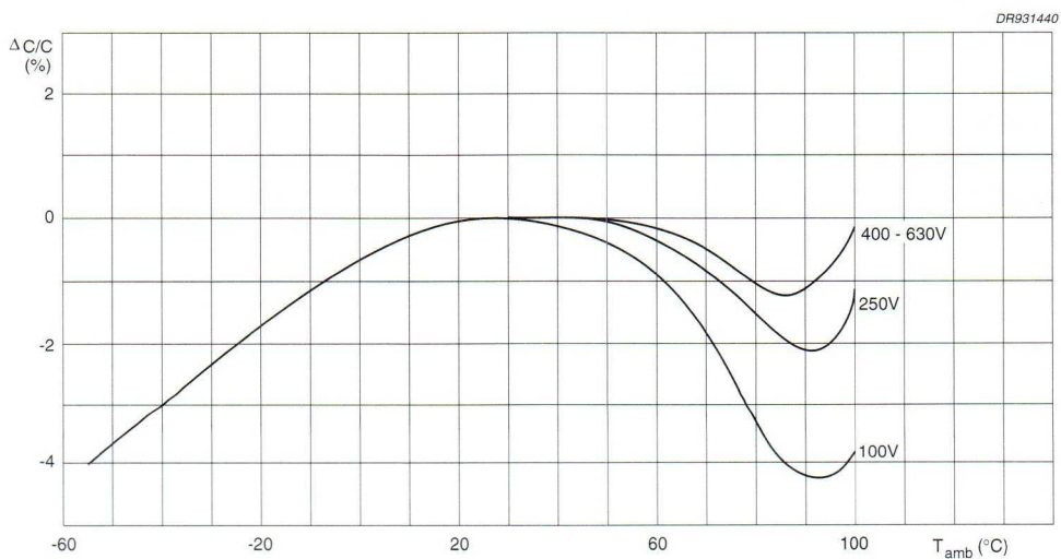
Fig.23 Capacitance as a function of ambient free air temperature, measured at 1 kHz, 1 V; typical curves.
