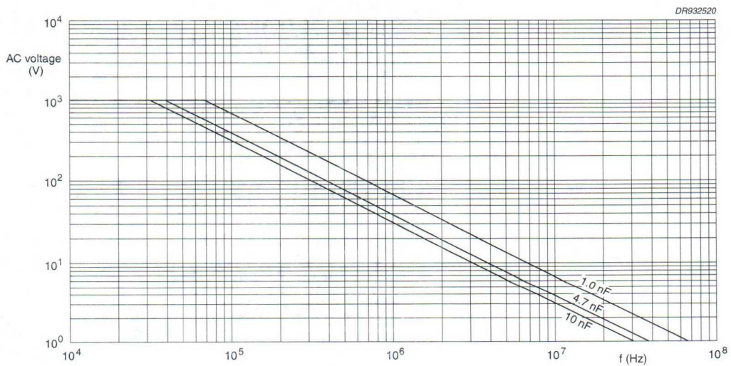
Fig.22 AC voltage (RMS value) as a function of frequency at T_{amb} \leq 70^\circ\text{C} for U_{Rdc} = 4000\text{ V} .
