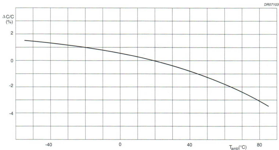
Fig.9 Capacitance change as a function of temperature; typical curve.
