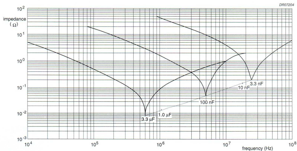
Fig.15 Impedance as a function of frequency; typical curves.
