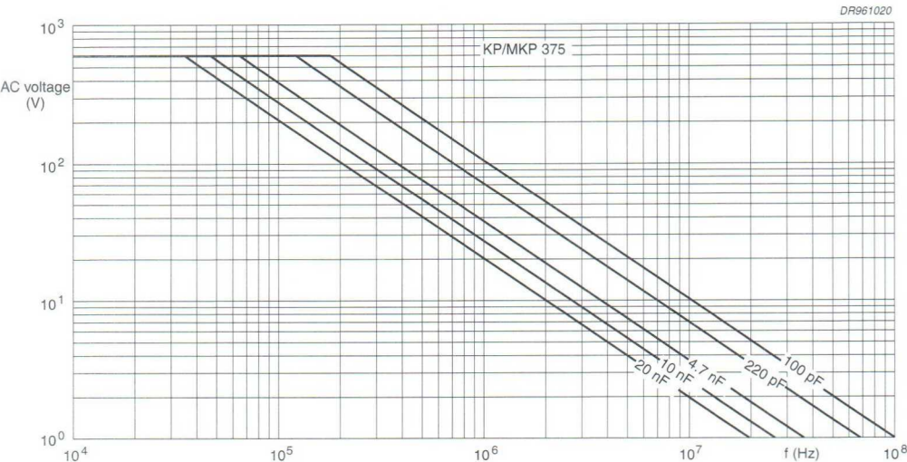
Fig.20 AC voltage (RMS value) as a function of frequency at T_{amb} \leq 85^\circ\text{C} for U_{Rdc} = 2000\text{ V} .
