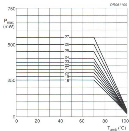
Fig.33 Maximum permissible power dissipation as a function of ambient temperature, at various capacitor dimensions.
