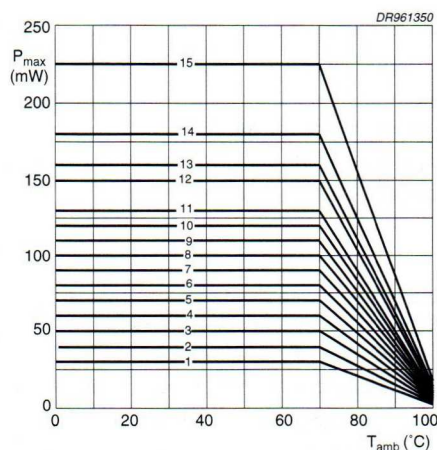
Fig.38 Maximum permissible power dissipation as a function of ambient temperature, at various capacitor dimensions.
