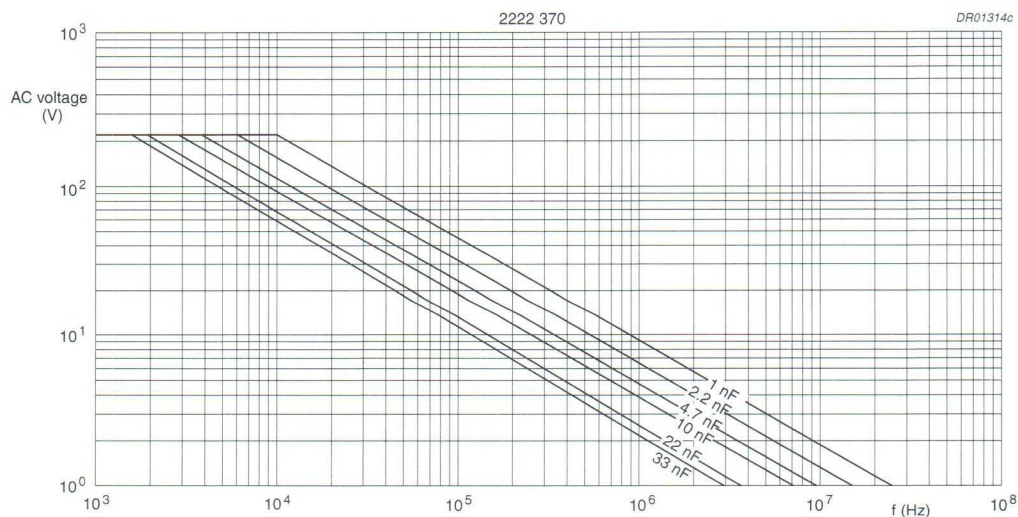
Fig.24 AC voltage (RMS value) as a function of frequency at T_{amb} \leq 85^\circ\text{C} for U_{Rdc} = 400\text{ V} .
