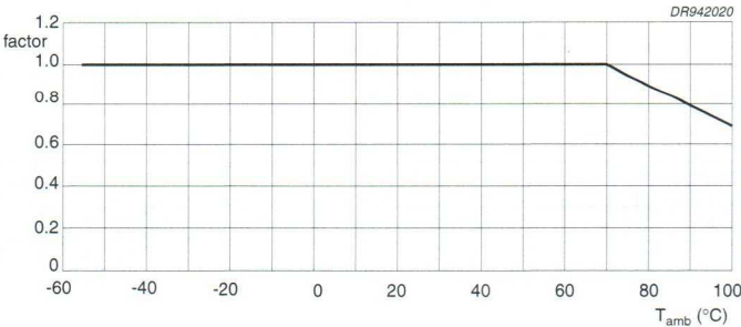
Fig.17 Multiplying factor as a function of temperature.
