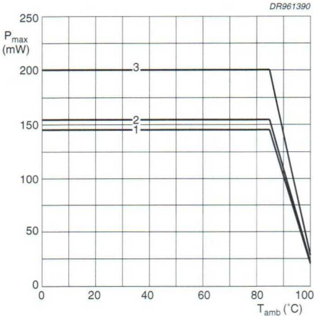
Fig.19 Maximum permissible power dissipation as a function of ambient temperature, at various capacitor dimensions.
