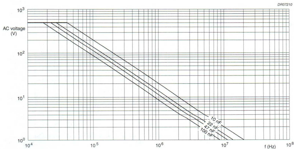
Fig.18 AC voltage (RMS value) as a function of frequency at T_{amb} \leq 70^\circ\text{C} for U_{Rdc} = 1600\text{ V} .
