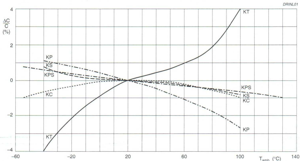
Fig.1 Capacitance change as a function of ambient free air temperature at 1 kHz; typical curves.
