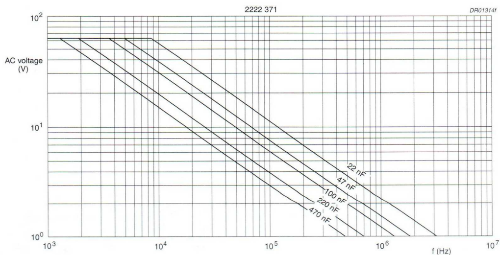
Fig.26 AC voltage (RMS value) as a function of frequency at T_{amb} \leq 85^\circ\text{C} for U_{Rdc} = 100\text{ V} .
