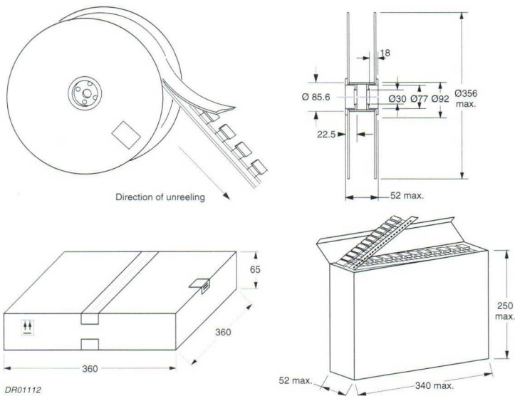
Fig.34 Outlines of reel and ammopack. Styles: 365, 374, 465, 466 and 479.
