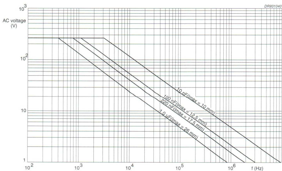
Fig.28 AC voltage (RMS value) as a function of frequency at T_{amb} \leq 85^\circ\text{C} for U_{Rdc} = 630\text{ V} .
