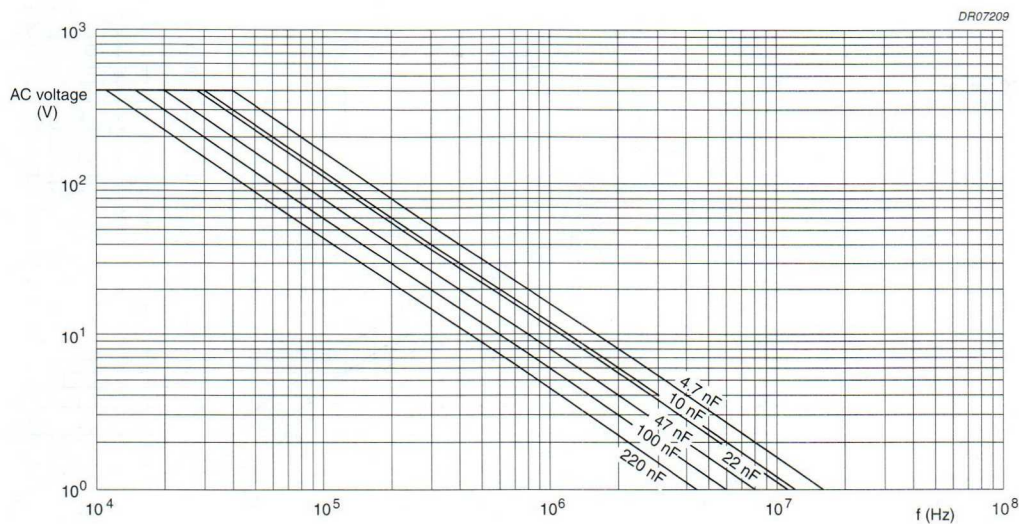
Fig.17 AC voltage (RMS value) as a function of frequency at T_{amb} \leq 70^\circ\text{C} for U_{Rdc} = 1000\text{ V} .
