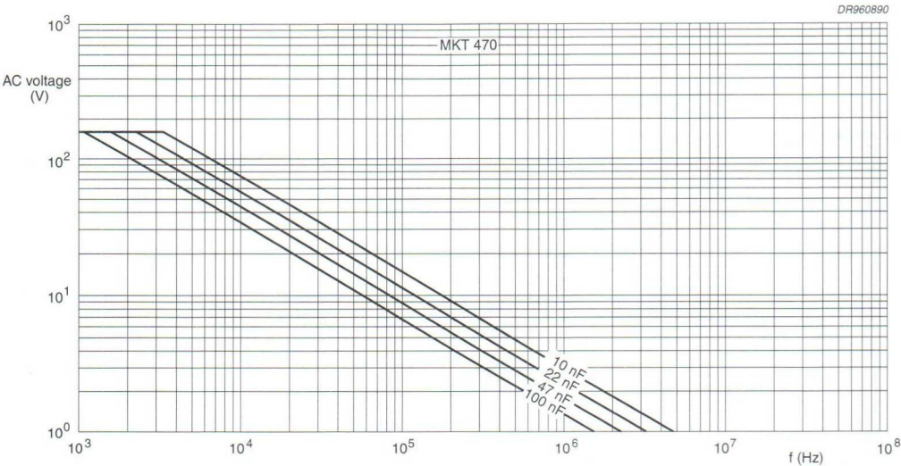
Fig.13 AC voltage (RMS value) as a function of frequency at T_{amb} \leq 85^\circ\text{C} for U_{Rdc} = 250\text{ V} .
