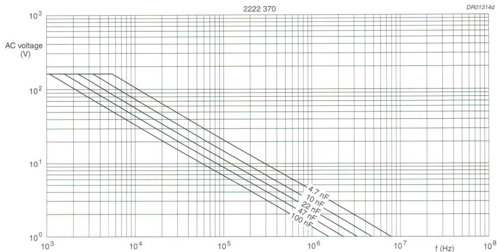
Fig.23 AC voltage (RMS value) as a function of frequency at T_{amb} \leq 85^\circ\text{C} for U_{Rdc} = 250\text{ V} .
