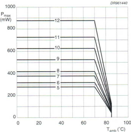
Fig.28 Maximum permissible power dissipation as a function of ambient temperature, at various capacitor dimensions.
