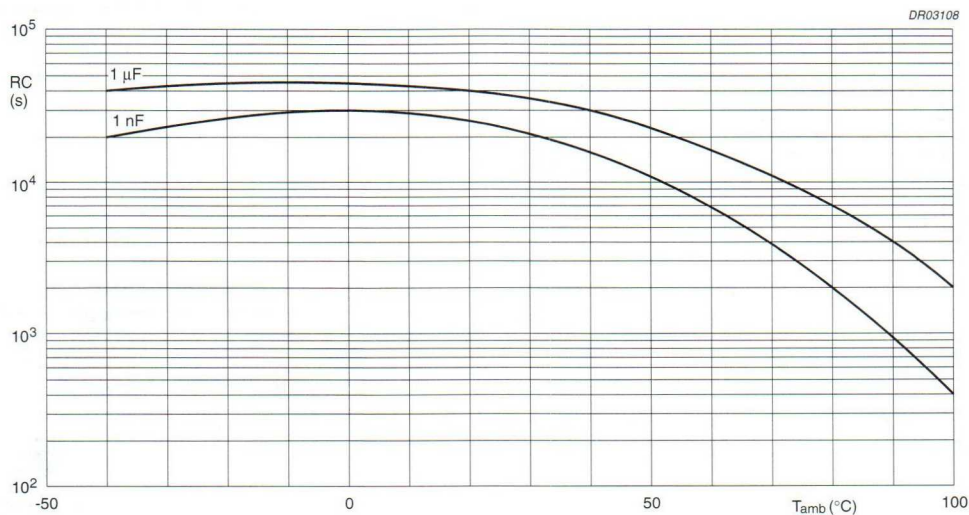
Fig.11 RC-product as a function of ambient free air temperature; typical curves.
