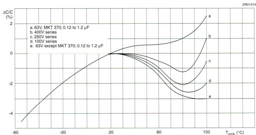
Fig.19 Capacitance change as a function of ambient free air temperature; typical curves.
