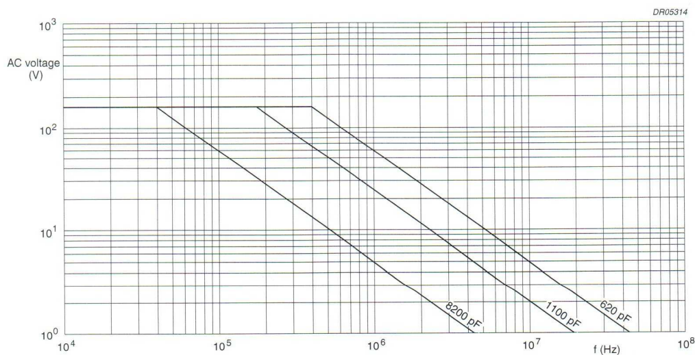
Fig.14 AC voltage (RMS value) as a function of frequency at T_{amb} \leq 70^\circ\text{C} for U_{Rdc} = 400\text{ V} .
