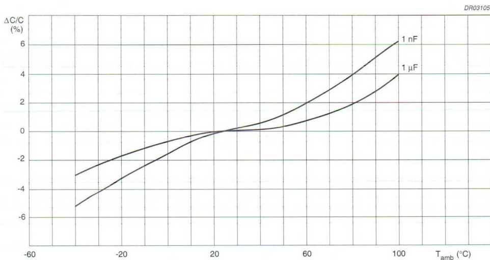
Fig.8 Capacitance change as a function of ambient free air temperature at 1 kHz; typical curves.
