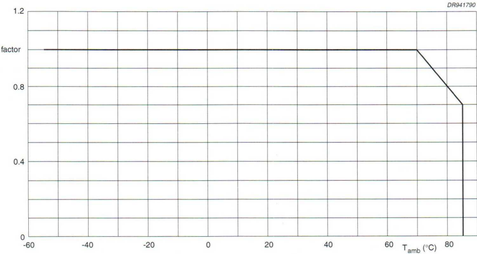
Fig.28 Multiplying factor as a function of temperature.
