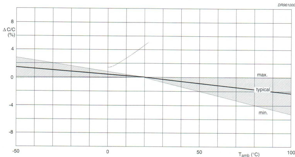
Fig.15 Capacitance change as a function of ambient temperature; typical curve.
