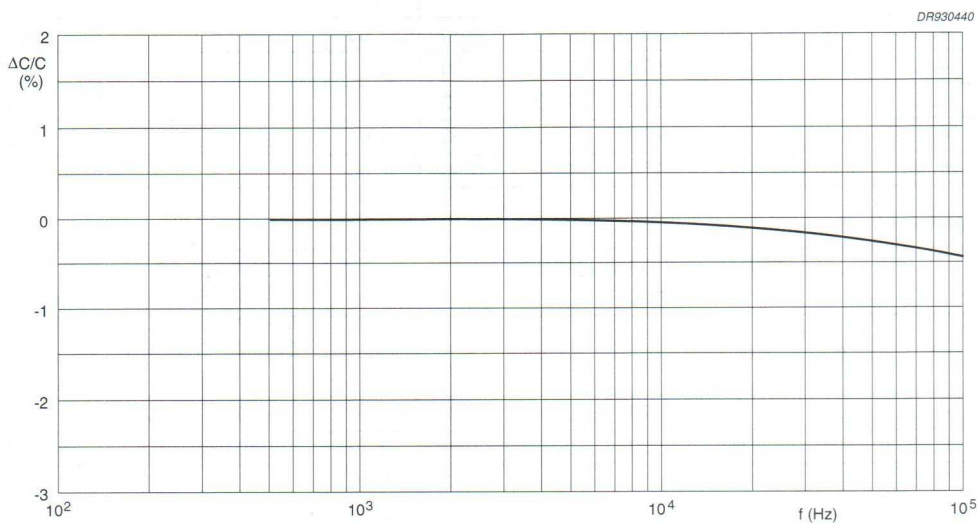
Fig.8 Capacitance change as a function of frequency; typical curve.
