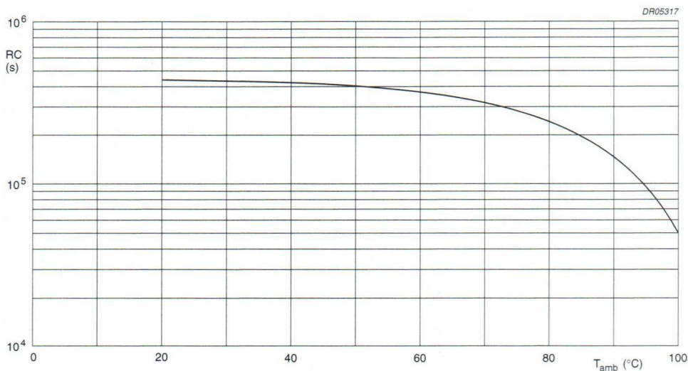
Fig.17 RC-product as a function of ambient free air temperature; typical curve.
