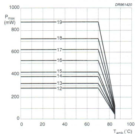
Fig.32 Maximum permissible power dissipation as a function of ambient temperature, at various capacitor dimensions.
