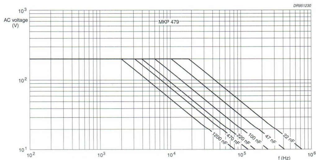
Fig.15 AC voltage (RMS value) as a function of frequency at T_{amb} \leq 70^\circ\text{C} for U_{Rdc} = 400\text{ V} .
