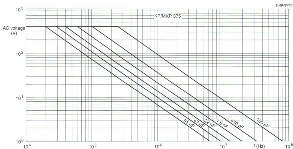
Fig.18 AC voltage (RMS value) as a function of frequency at T_{amb} \leq 85^\circ\text{C} for U_{Rdc} = 1000\text{ V} .
