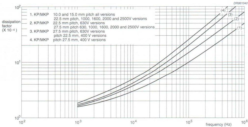
Fig.24 Tangent of loss angle as a function of frequency; maximum curves.
