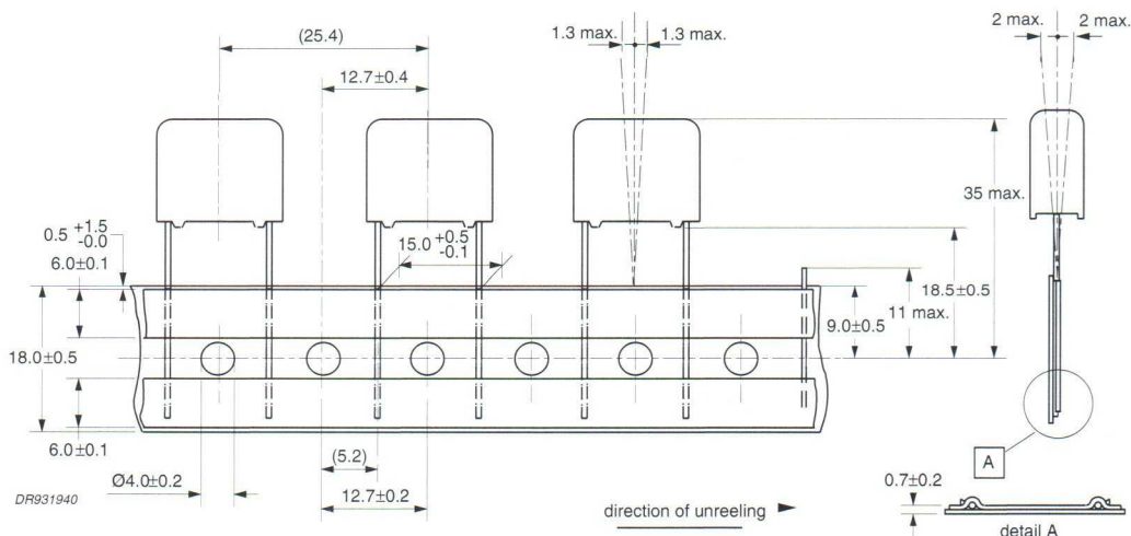
Fig.14 Outline of taped capacitors: pitch = 15 mm.
