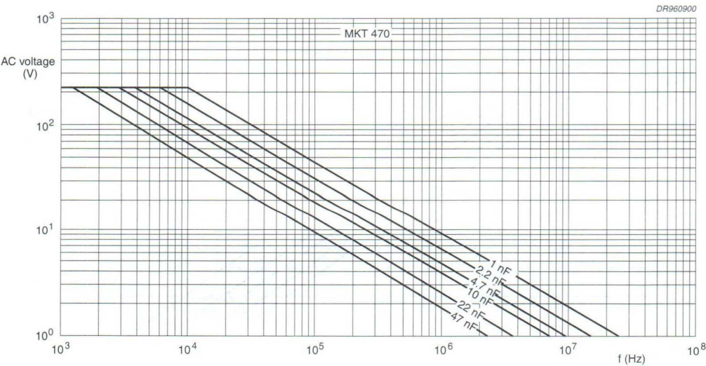
Fig.14 AC voltage (RMS value) as a function of frequency at T_{amb} \leq 85^\circ\text{C} for U_{Rdc} = 400\text{ V} .
