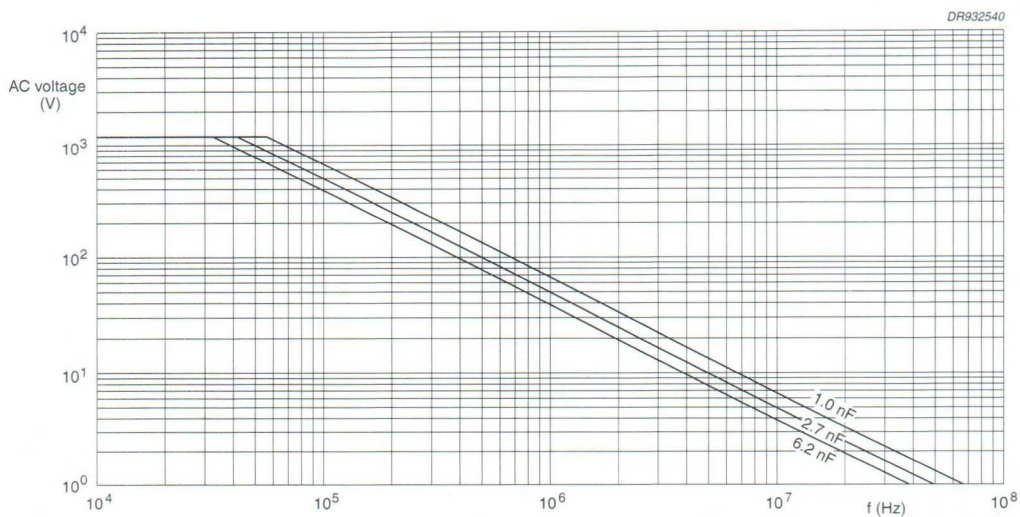
Fig.23 AC voltage (RMS value) as a function of frequency at T_{amb} \leq 70^\circ\text{C} for U_{Rdc} = 5000\text{ V} .
