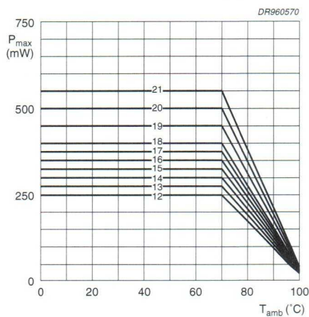
Fig.13 Maximum dissipation as a function of ambient free air temperature, at various capacitor dimensions.
