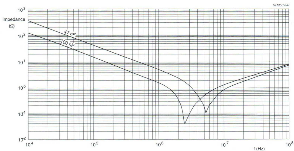
Fig.8 Impedance as a function of frequency; typical curves.
