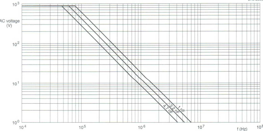
Fig.21 AC voltage (RMS value) as a function of frequency at T_{amb} \leq 85^\circ\text{C} for U_{Rdc} = 2500\text{ V} .
