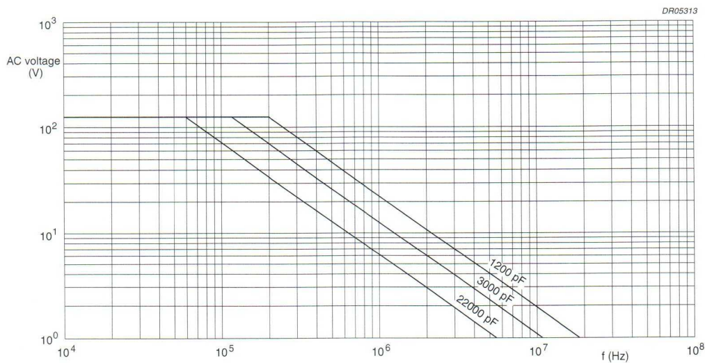
Fig.13 AC voltage (RMS value) as a function of frequency at T_{amb} \leq 70^\circ\text{C} for U_{Rdc} = 250\text{ V} .
