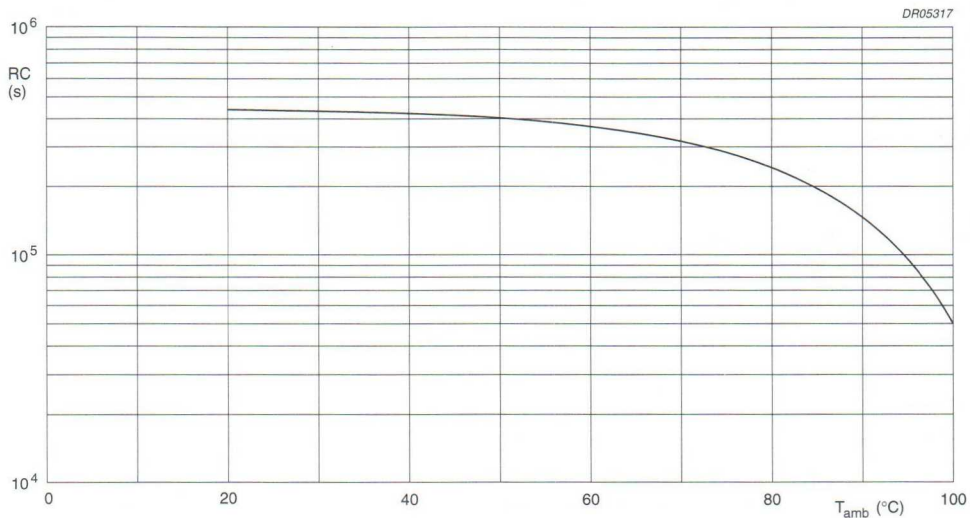
Fig.25 RC product as a function of ambient temperature: typical curve.
