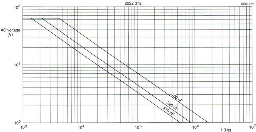
Fig.29 AC voltage (RMS value) as a function of frequency at T_{amb} \leq 85^\circ\text{C} for U_{Rdc} = 100\text{ V} .
