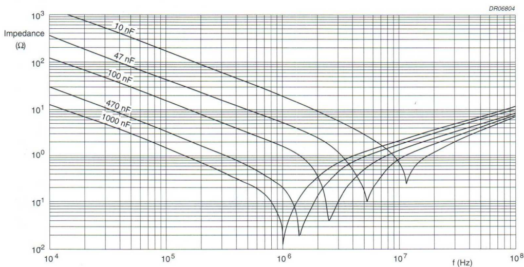
Fig.7 Impedance as a function of frequency; typical curves.
