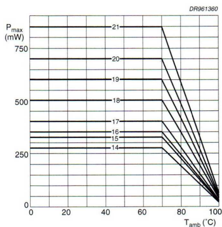
Fig.39 Maximum permissible power dissipation as a function of ambient temperature, at various capacitor dimensions.
