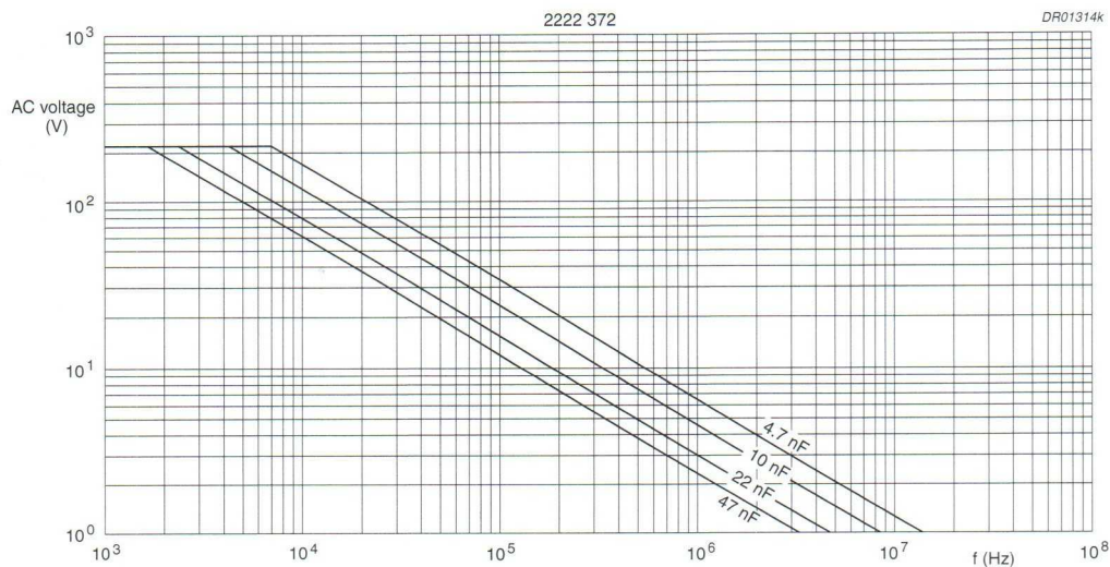
Fig.31 AC voltage (RMS value) as a function of frequency at T_{amb} \leq 85^\circ\text{C} for U_{Rdc} = 400\text{ V} .
