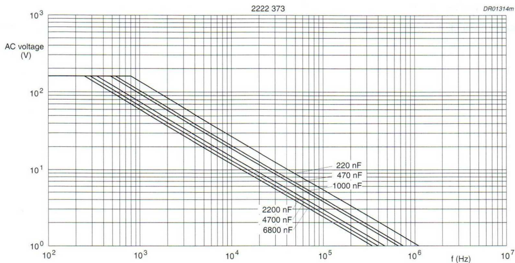
Fig.33 AC voltage (RMS value) as a function of frequency at T_{amb} \leq 85^\circ\text{C} for U_{Rdc} = 250\text{ V} .
