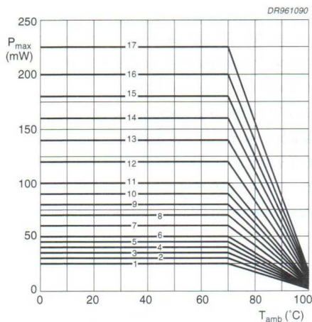
Fig.32 Maximum permissible power dissipation as a function of ambient temperature, at various capacitor dimensions.
