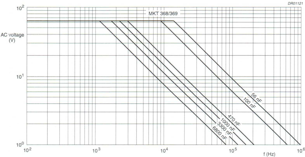
Fig.39 AC voltage (RMS value) as a function of frequency at T_{amb} \leq 85^\circ\text{C} , for U_{Rdc} = 100\text{ V} (2222 368 and 369 styles).
