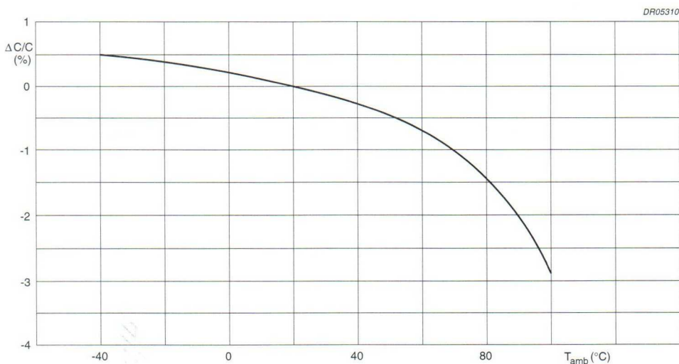
Fig.10 Capacitance as a function of ambient temperature; typical curve.
