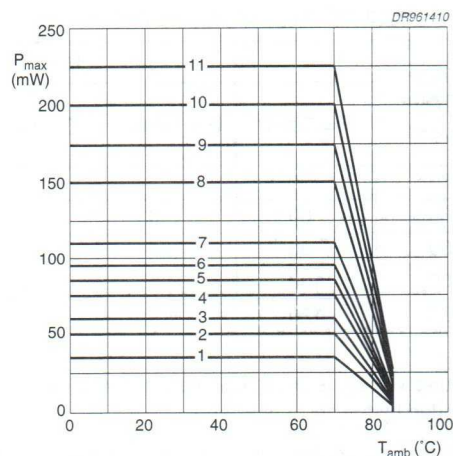
Fig.31 Maximum permissible power dissipation as a function of ambient temperature, at various capacitor dimensions.
