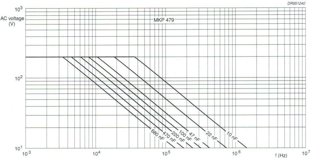
Fig.16 AC voltage (RMS value) as a function of frequency at T_{amb} \leq 70\text{ }^{\circ}\text{C} for U_{Rdc} = 630\text{ V} .
