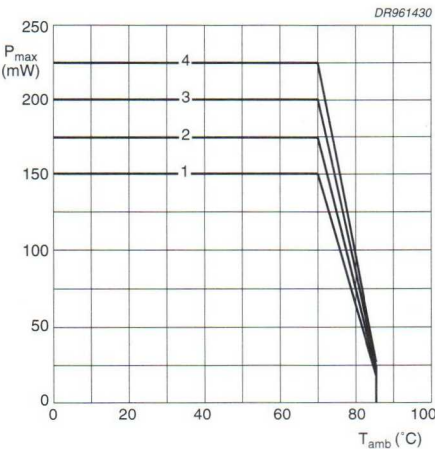
Fig.27 Maximum permissible power dissipation as a function of ambient temperature, at various capacitor dimensions.
