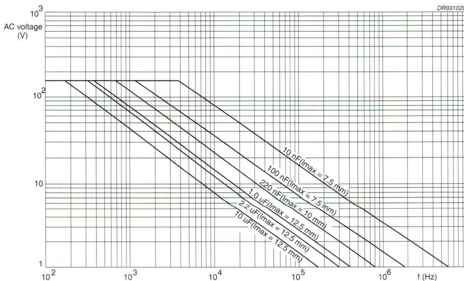
Fig.26 AC voltage (RMS value) as a function of frequency at T_{amb} \leq 85^\circ\text{C} for U_{Rdc} = 250\text{ V} .
