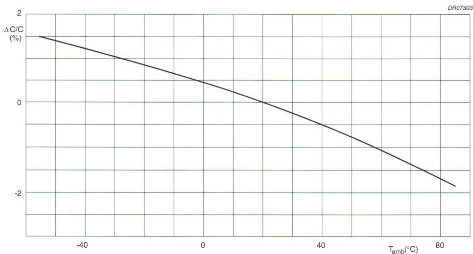
Fig.17 Capacitance change as a function of temperature; typical curve.
