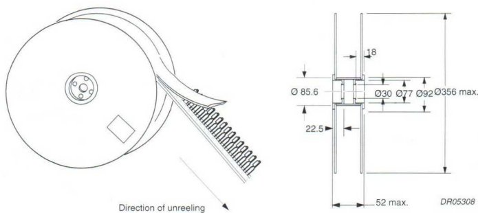
Fig.4 Outline of tape mounted on reel.
