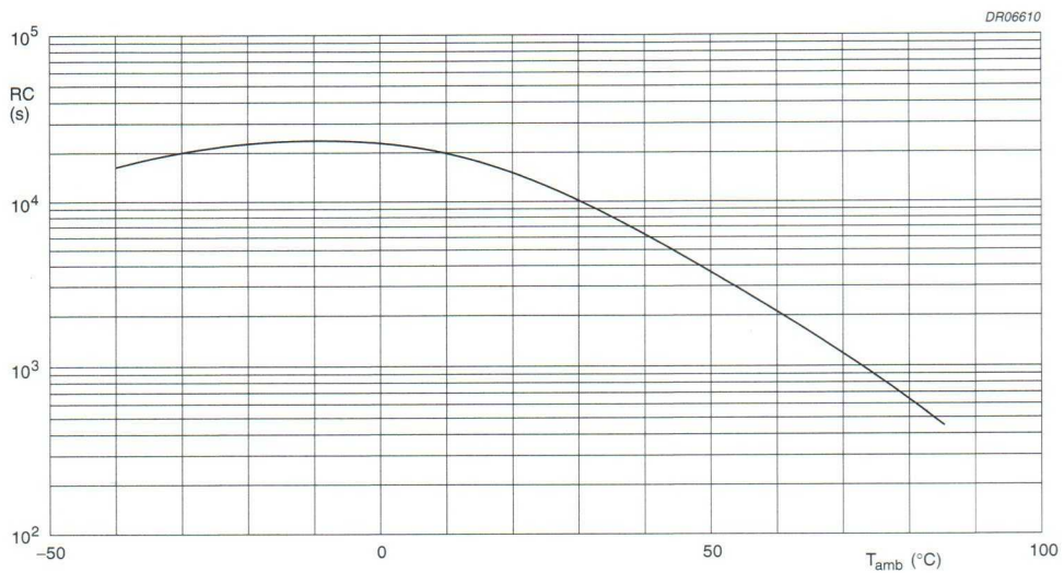
Fig.11 RC product as a function of ambient free air temperature; typical curve.
