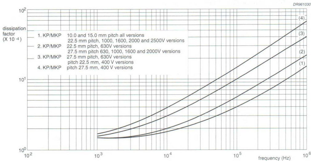
Fig.23 Tangent of loss angle as a function of frequency; typical curves.
