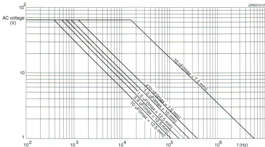
Fig.25 AC voltage (RMS value) as a function of frequency at T_{amb} \leq 85^\circ\text{C} for U_{Rdc} = 100\text{ V} .
