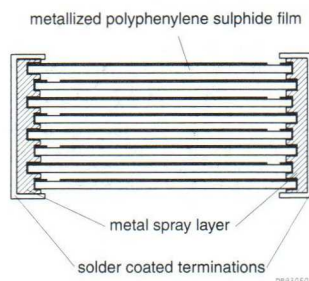
Fig.3 Construction.
