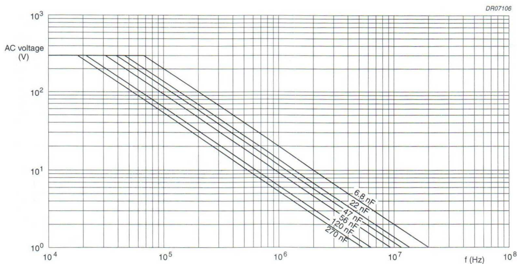
Fig.12 AC voltage (RMS value) as a function of frequency at T_{amb} \leq 85^\circ\text{C} for U_{Rdc} = 630\text{ V} .
