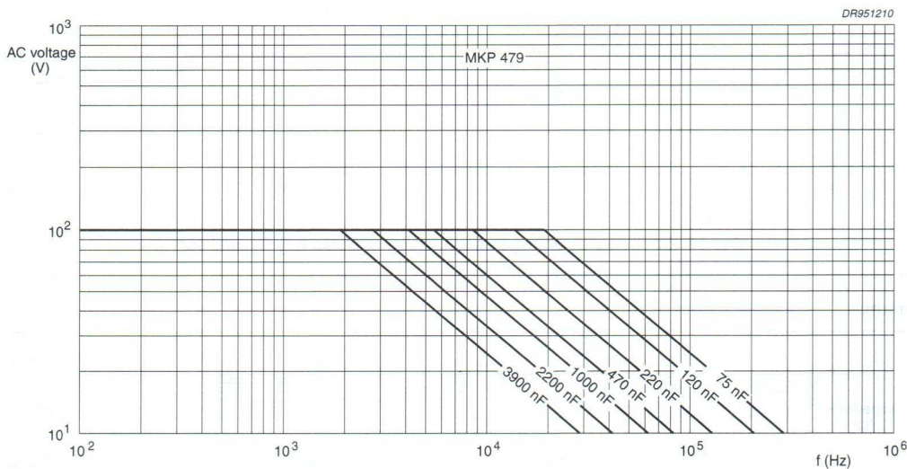
Fig.13 AC voltage (RMS value) as a function of frequency at T_{\text{amb}} \leq 70\text{ }^{\circ}\text{C} for U_{\text{Rdc}} = 160\text{ V} .
