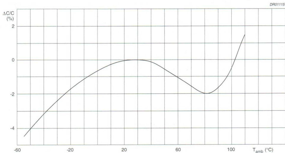
Fig.32 Capacitance as a function of ambient free air temperature; typical curve.
