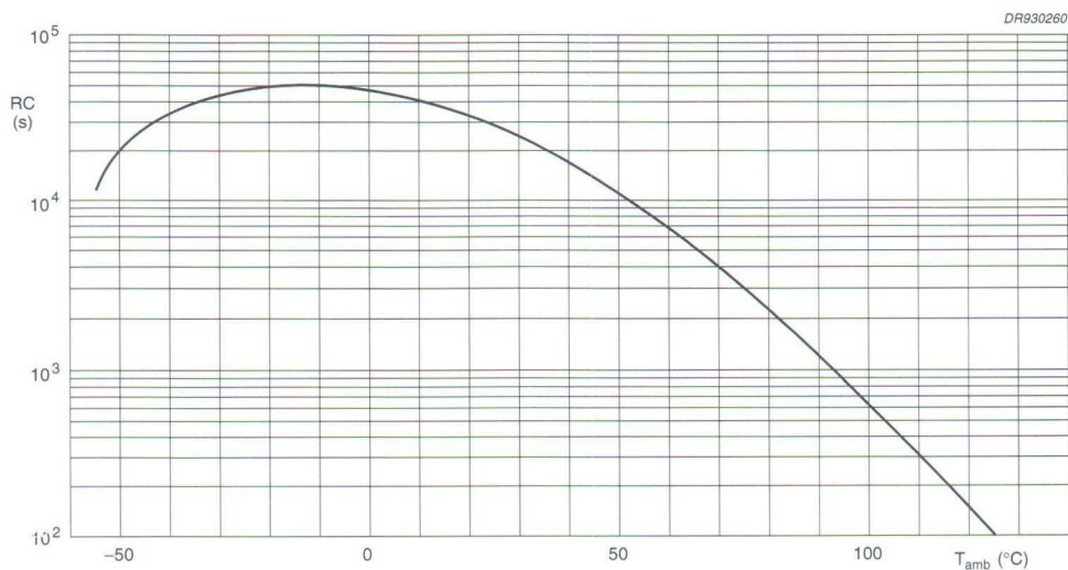
Fig.17 RC product as a function of temperature; typical curve.
