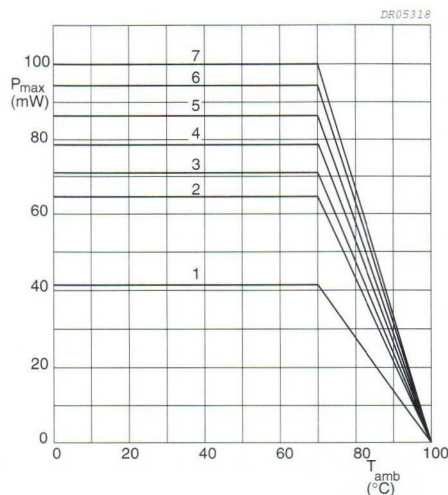
Fig.19 Maximum dissipation as a function of ambient temperature.
