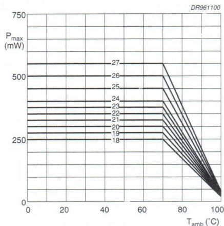
Fig.21 Maximum permissible power dissipation as a function of ambient temperature, at various capacitor dimensions for 630 V series.
