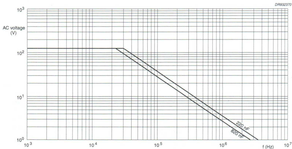
Fig.11 AC voltage (RMS value) as a function of frequency at T_{\text{amb}} \leq 85 \text{ }^{\circ}\text{C} for U_{\text{Rdc}} = 250 \text{ V} .
