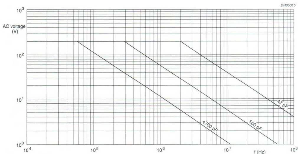
Fig.15 AC voltage (RMS value) as a function of frequency at T_{amb} \leq 70^\circ\text{C} for U_{Rdc} = 630\text{ V} .
