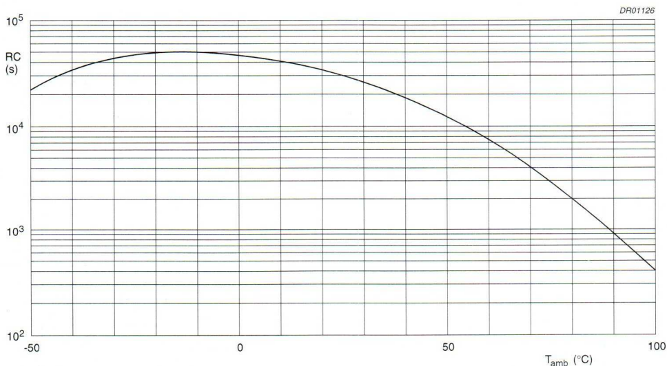
Fig.31 RC product as a function of ambient free air temperature; typical curve.
