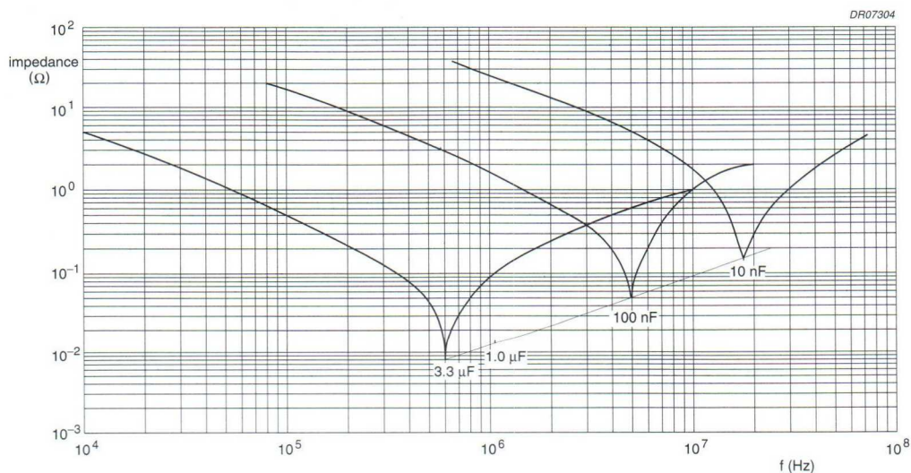
Fig.12 Impedance as a function of frequency; typical curves.
