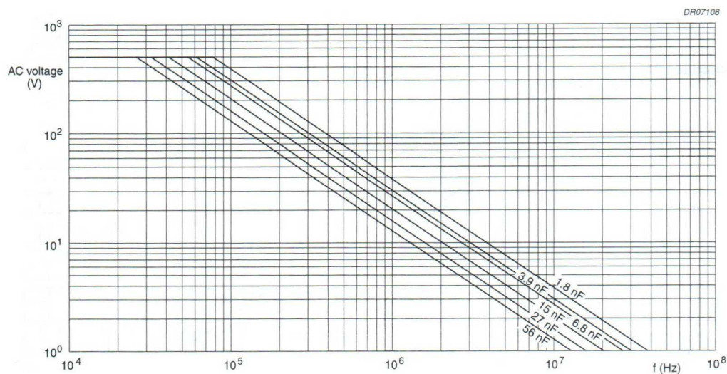
Fig.14 AC voltage (RMS value) as a function of frequency at T_{amb} \leq 85^\circ\text{C} for U_{Rdc} = 1600\text{ V} .
