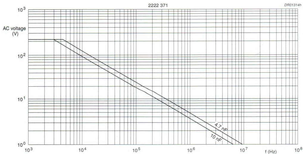
Fig.28 AC voltage (RMS value) as a function of frequency at T_{amb} \leq 85^\circ\text{C} for U_{Rdc} = 400\text{ V} .
