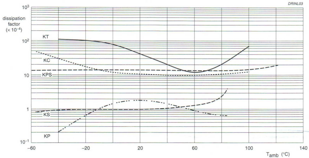
Fig.3 Dissipation factor as a function of ambient free air temperature at 1 kHz; typical curves.
