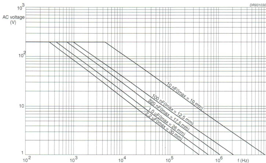
Fig.27 AC voltage (RMS value) as a function of frequency at T_{amb} \leq 85^\circ\text{C} for U_{Rdc} = 400\text{ V} .
