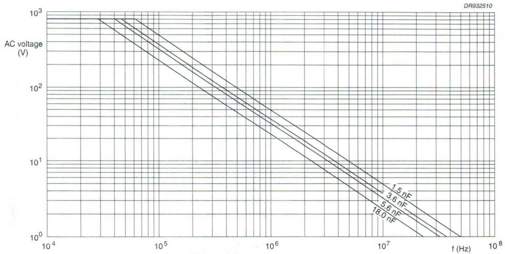
Fig.21 AC voltage (RMS value) as a function of frequency at T_{amb} \leq 70^\circ\text{C} for U_{Rdc} = 3000\text{ V} .
