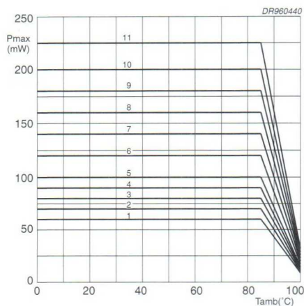
Fig.26 Maximum dissipation as a function of ambient free air temperature, at various capacitor dimensions.
