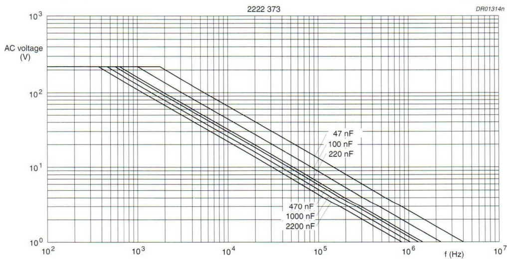
Fig.34 AC voltage (RMS value) as a function of frequency at T_{amb} \leq 85^\circ\text{C} for U_{Rdc} = 400\text{ V} .
