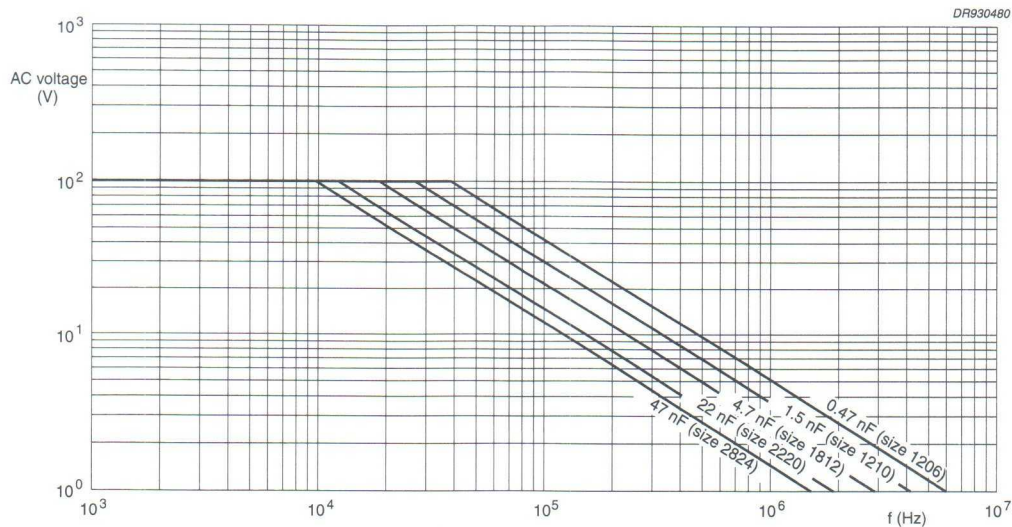
Fig.13 Maximum AC voltage as a function of frequency: U_{Rdc} = 160 \text{ V} .
