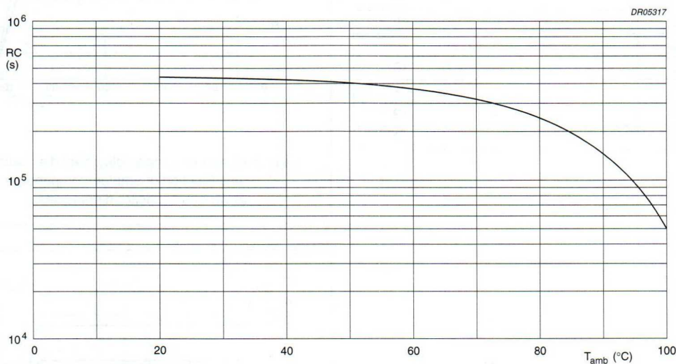
Fig.18 RC product as a function of ambient temperature; typical curve.
