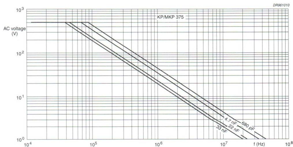
Fig.19 AC voltage (RMS value) as a function of frequency at T_{amb} \leq 85^\circ\text{C} for U_{Rdc} = 1600\text{ V} .
