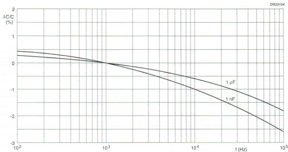
Fig.7 Capacitance change as a function of frequency; typical curves.
