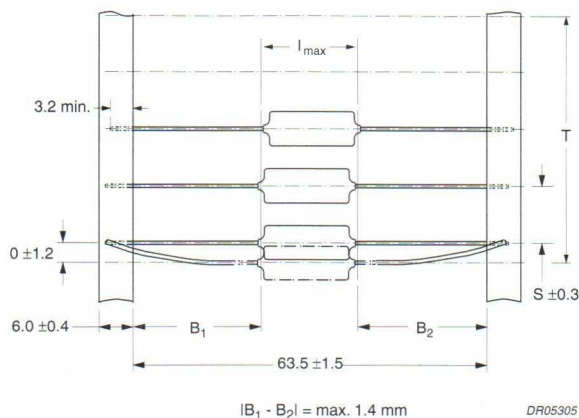
Fig.5 Outline of axial taped capacitors. Tape distance: 63.5 \pm 1.5 mm.
