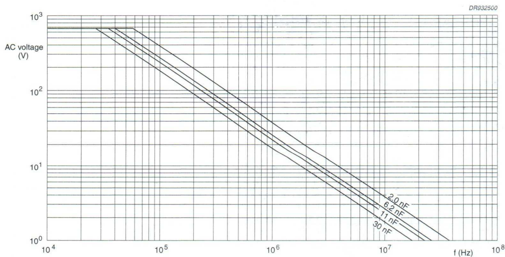
Fig.20 AC voltage (RMS value) as a function of frequency at T_{\text{amb}} \leq 70^\circ\text{C} for U_{\text{Rdc}} = 2500\text{ V} .
