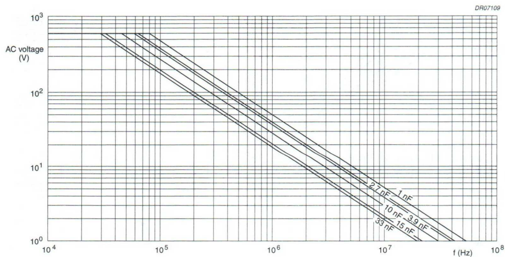
Fig.15 AC voltage (RMS value) as a function of frequency at T_{amb} \leq 85^\circ\text{C} for U_{Rdc} = 2000\text{ V} .
