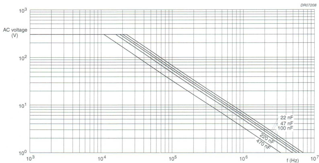
Fig.16 AC voltage (RMS value) as a function of frequency at T_{amb} \leq 70 °C for U_{Rdc} = 630 V.
