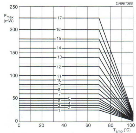
Fig.18 Maximum permissible power dissipation as a function of ambient temperature, at various capacitor dimensions for 200 and 250 V series.
