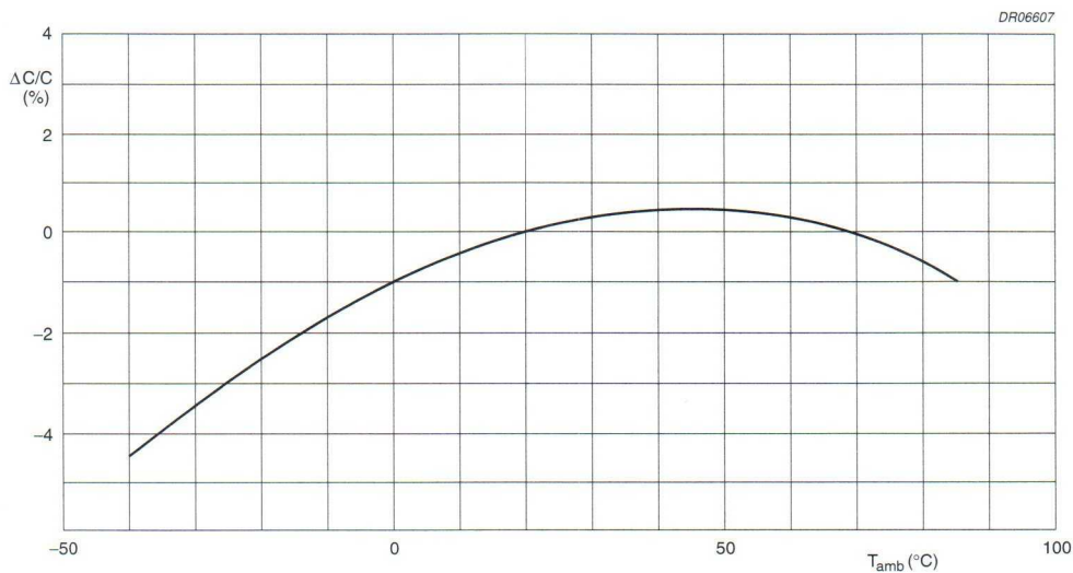
Fig.6 Capacitance change as a function of ambient temperature; typical curve.
