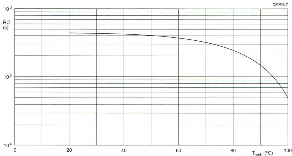
Fig.19 RC product as a function of ambient free air temperature; typical curve.
