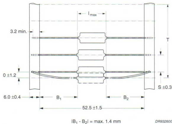
Fig.6 Outline of axial taped capacitors. Tape distance: 52.5 \pm 1.5 mm.
