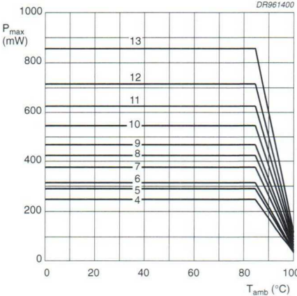
Fig.20 Maximum permissible power dissipation as a function of ambient temperature, at various capacitor dimensions.
