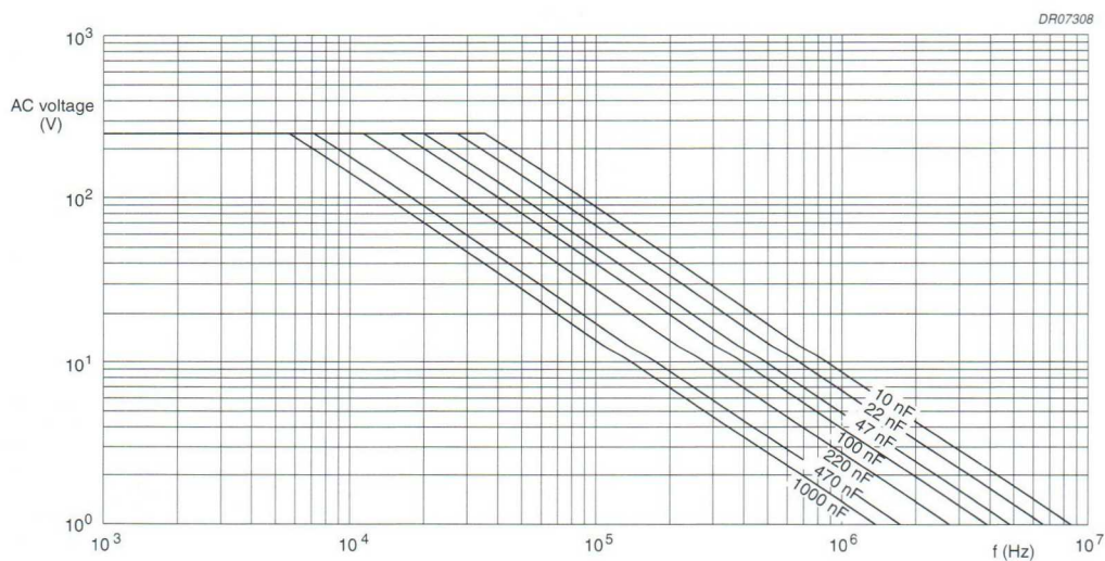
Fig.27 AC voltage (RMS value) as a function of frequency at T_{\text{amb}} \leq 70^\circ\text{C} for U_{\text{Rdc}} = 630\text{ V} .
