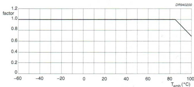
Fig.15 Multiplying factor as a function of temperature.
