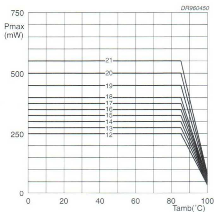
Fig.27 Maximum dissipation as a function of ambient free air temperature, at various capacitor dimensions.
