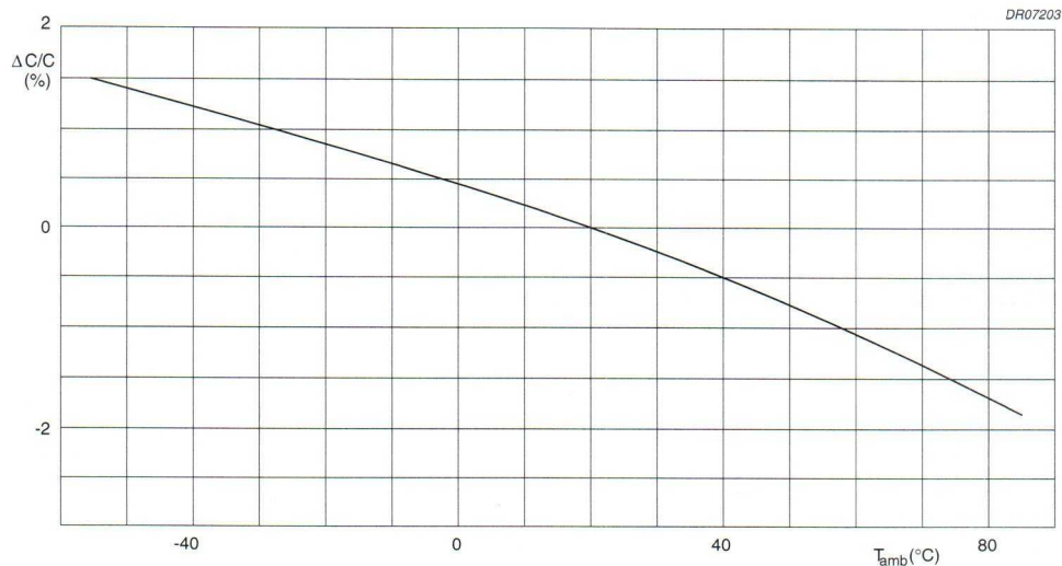
Fig.14 Capacitance change as a function of ambient temperature; typical curve.
