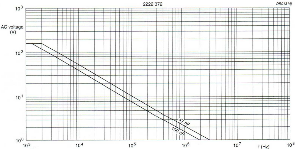
Fig.30 AC voltage (RMS value) as a function of frequency at T_{amb} \leq 85^\circ\text{C} for U_{Rdc} = 250\text{ V} .
