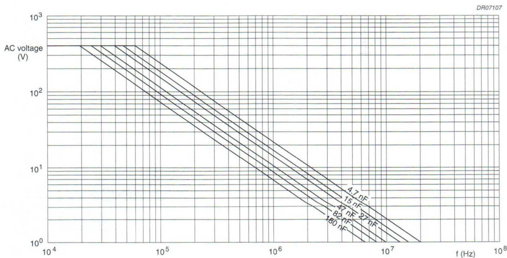
Fig.13 AC voltage (RMS value) as a function of frequency at T_{amb} \leq 85^\circ\text{C} for U_{Rdc} = 1000\text{ V} .
