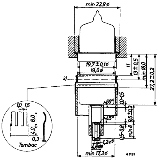
Fig. 30. Eccentricity. Distance between axes of the electrodes: g-a max. 0.38 mm; k-a max. 0.38 mm; f-k max. 0.12 mm.
