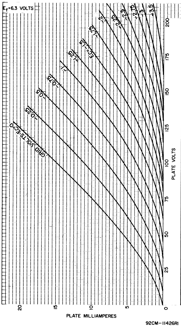
Fig.16 - Typical plate characteristics, type 8058.
