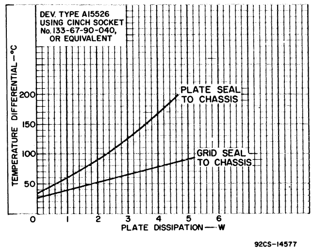
Fig. 24 - Temperature differentials, from plate seal to chassis and grid seal to chassis, as functions of plate dissipation, dev. type A15526.
