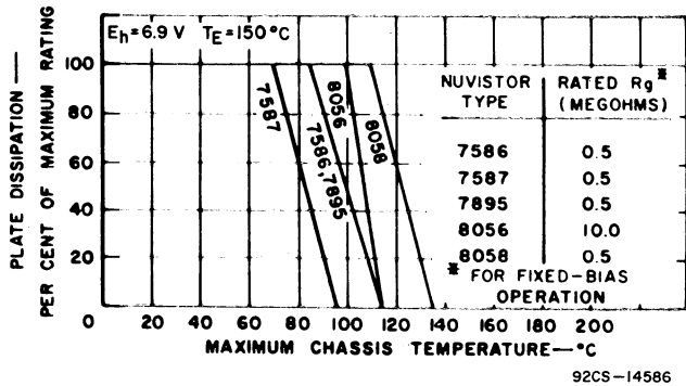
Fig. 4 - Combinations of plate dissipation and chassis temperature for metal-shell temperature of 150° C.
