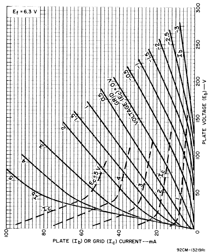
Fig.17 - Typical characteristics, type 8627.
