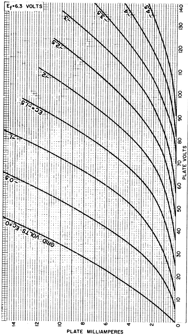
Fig. 7 - Typical plate characteristics, type 7586.
