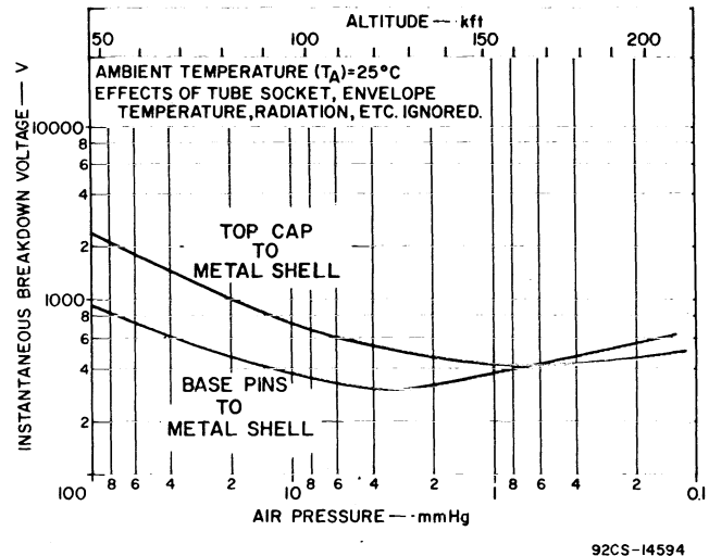
Fig. 6 - Breakdown-voltage characteristics, type 8627 and dev. type A15526.
