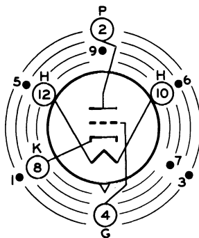
INDEX=LARGE LUG ●=SHORT PIN-IC JEDEC 12AQ
