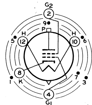
INDEX=LARGE LUG ●=SHORT PIN-IC JEDEC 12AS
