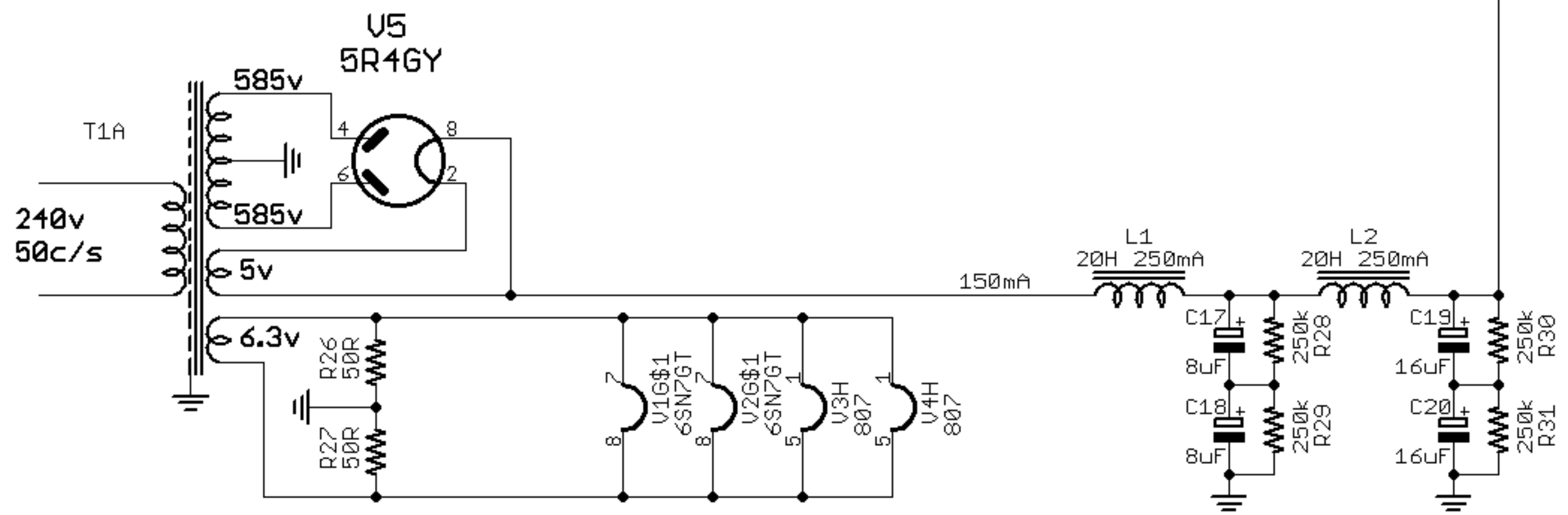
AWV RADIOTRON AMPLIFIER A515 Low Distortion Amplifier using 807 Triodes from RADIOTRONICS Nov/Dec, 1947, page 99 see also Mar/Apr 1948, inter-modulation tests
