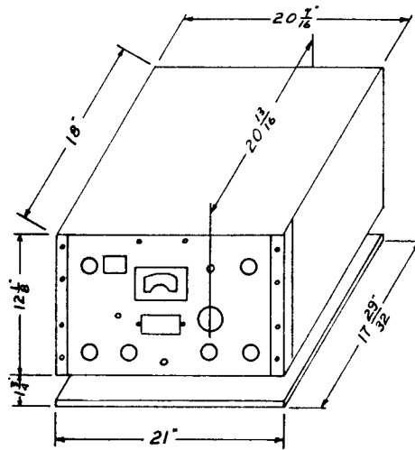
TYPE CZC-46209 RADIO RECEIVER WEIGHT 106 LBS.
