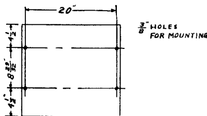
MOUNTING BASE
