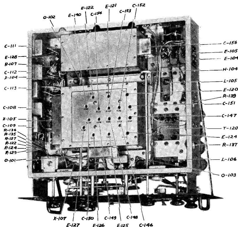
FIG. 2.111 LEFT BOTTOM OBLIQUE VIEW, RADIO RECEIVER CHASSIS
