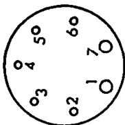
Hivac Five Pin (SM5)
